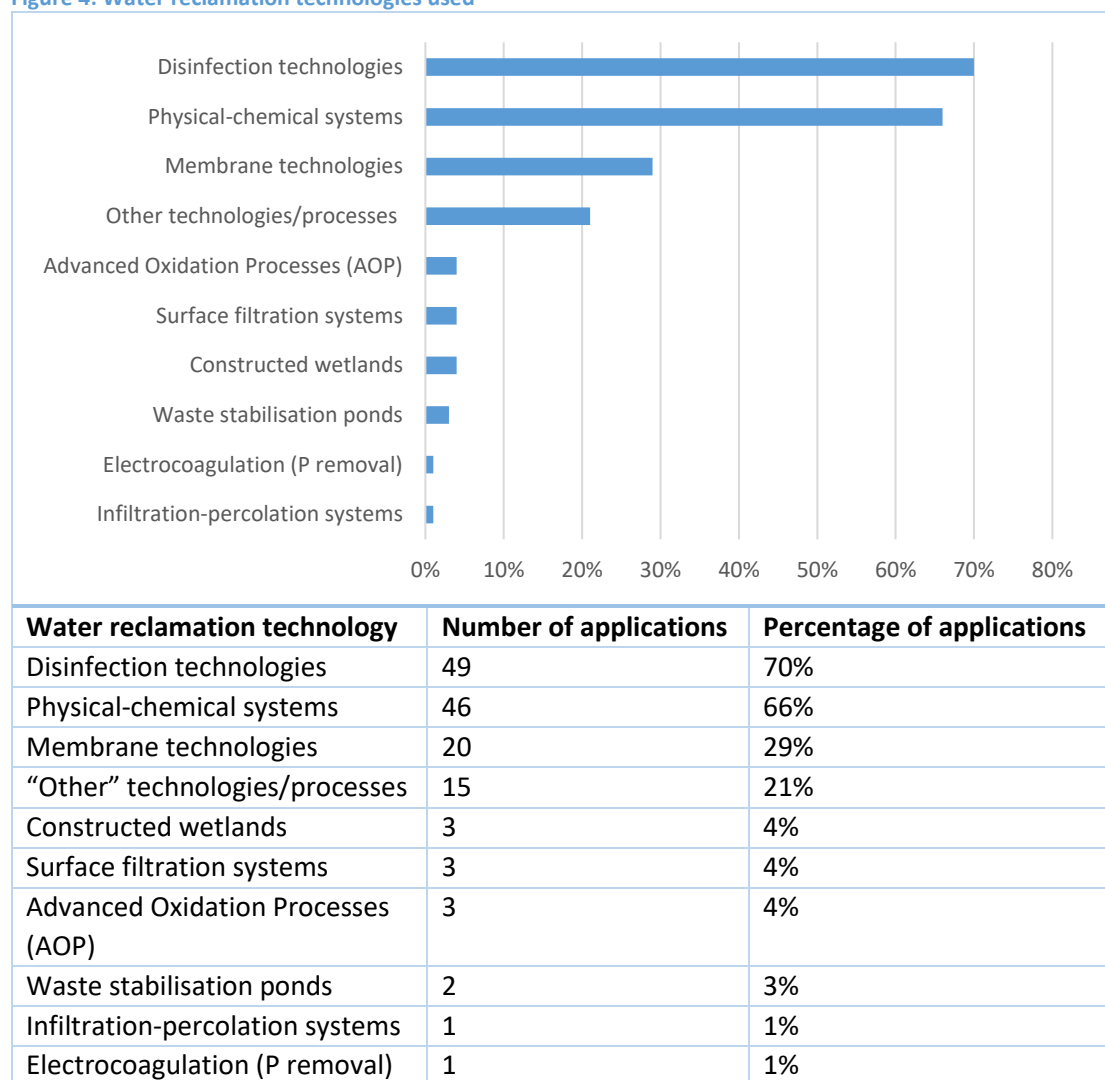
Figure 4: Water reclamation technologies used
